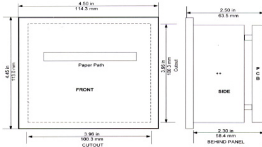
PL-180/PL-190 Series Impact Panel Mount Printer
